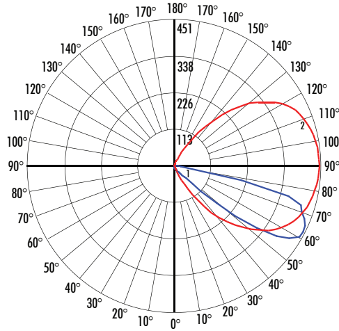
Maximum Candela = 451.17 Located At Horizontal Angle = 2.5, Vertical Angle = 62.5 # 1 - Vertical Plane Through Horizontal Angles (2.5 - 182.5) (Through Max. Cd.) # 2 - Horizontal Cone Through Vertical Angle (62.5) (Through Max. Cd.)
