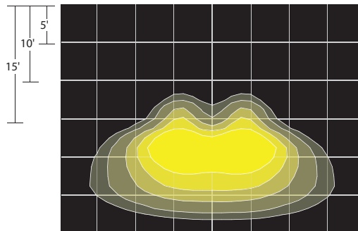
FOOTCANDLES ON GROUND 2 Fixture Overlap, 10 Ft. Spacing 3 Ft. Light Source Mtg. Ht., 1080 lm
