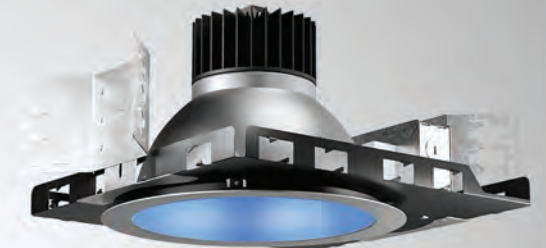
SR10 10" RGBW Recessed Downlight 1,450lm max. (48W)
