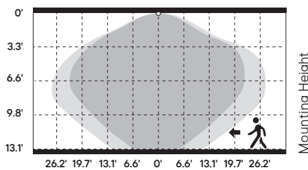
13' Height
