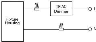
TRIAC
